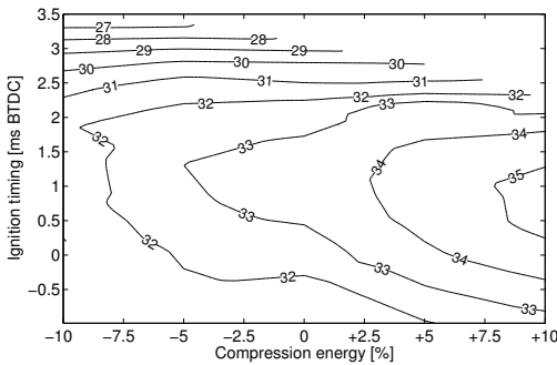
Fig. 9. Engine indicated efficiency (per cent) map for varying compression energy and spark timing.
