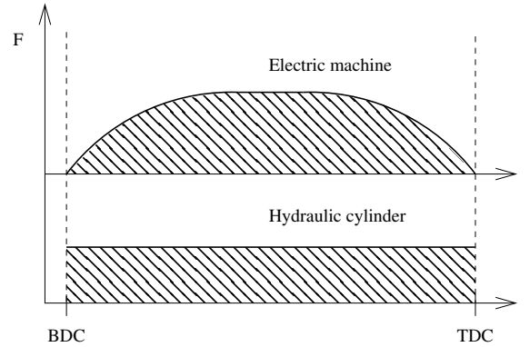
Fig. 5. Illustration of the force profiles of free-piston engine loads.
