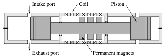
(b) Dual piston free-piston engine generator [3].
