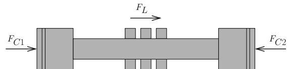
Fig. 3. Free body diagram of free-piston engine mover.
