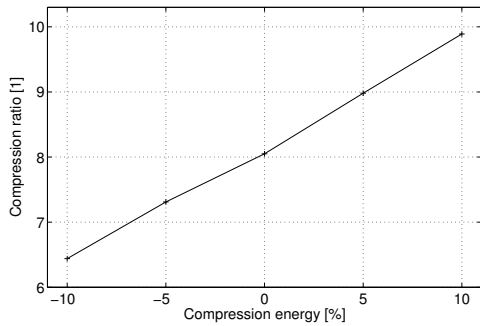
(b) Effect on engine compression ratio.
