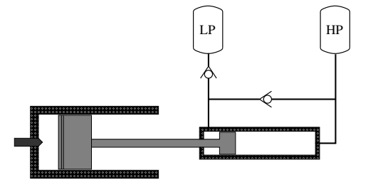
(a) Single piston hydraulic free-piston engine [2].
