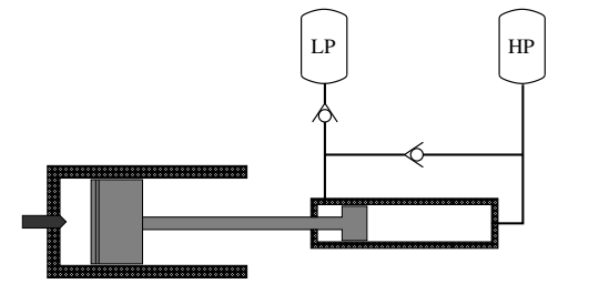
(a) Single piston hydraulic free-piston engine [2].
